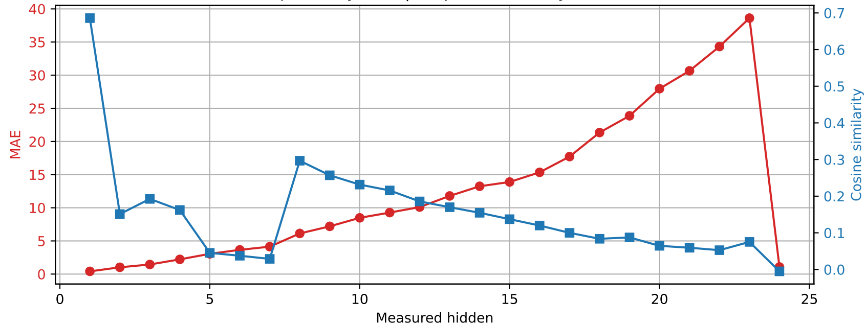
SmolLM2-1.7B-Instruct | Prompt 3 Spared layer 19 | Unquantized vs hybrid
