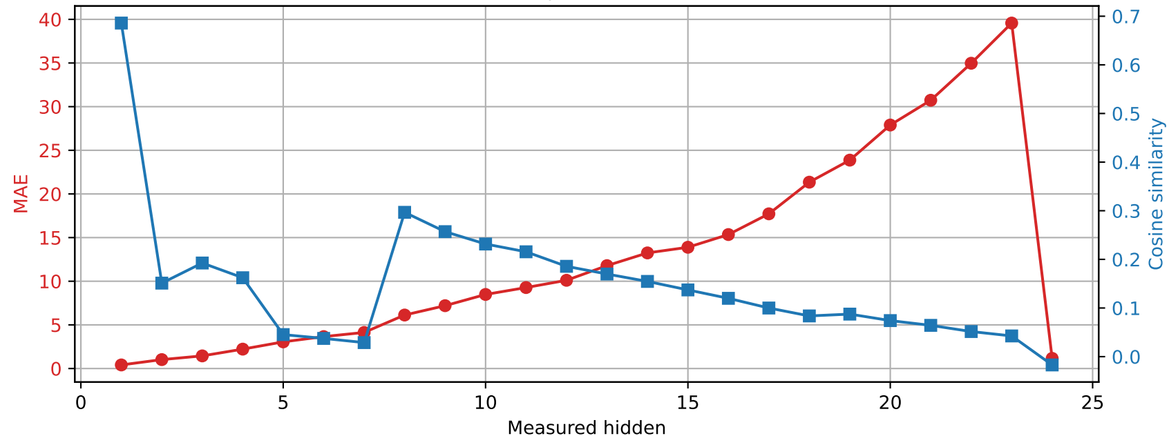
SmolLM2-1.7B-Instruct | Prompt 3 Spared layer 21 | Unquantized vs hybrid
