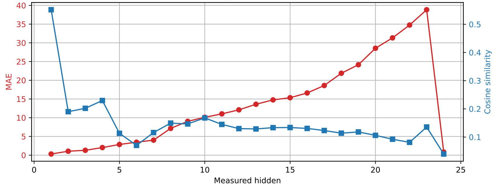
SmolLM2-1.7B-Instruct | Prompt 4 Spared layer 8 | Unquantized vs hybrid
