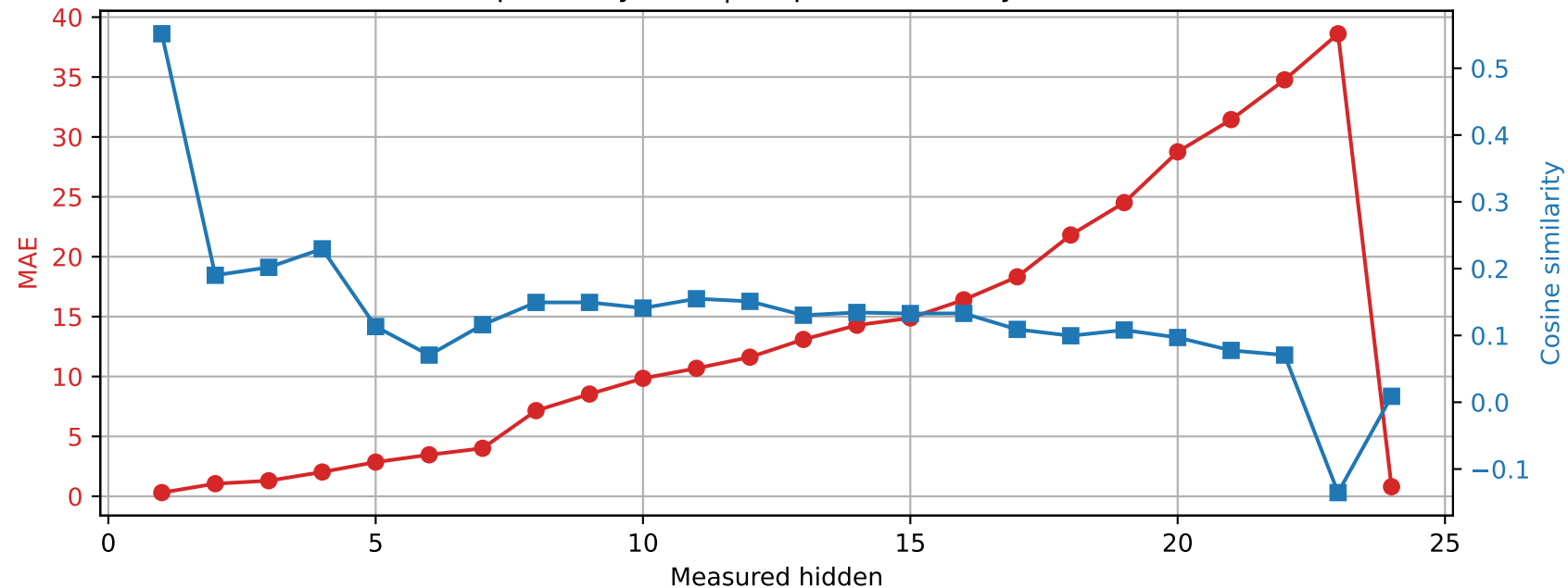
SmolLM2-1.7B-Instruct | Prompt 4 Spared layer 10 | Unquantized vs hybrid
