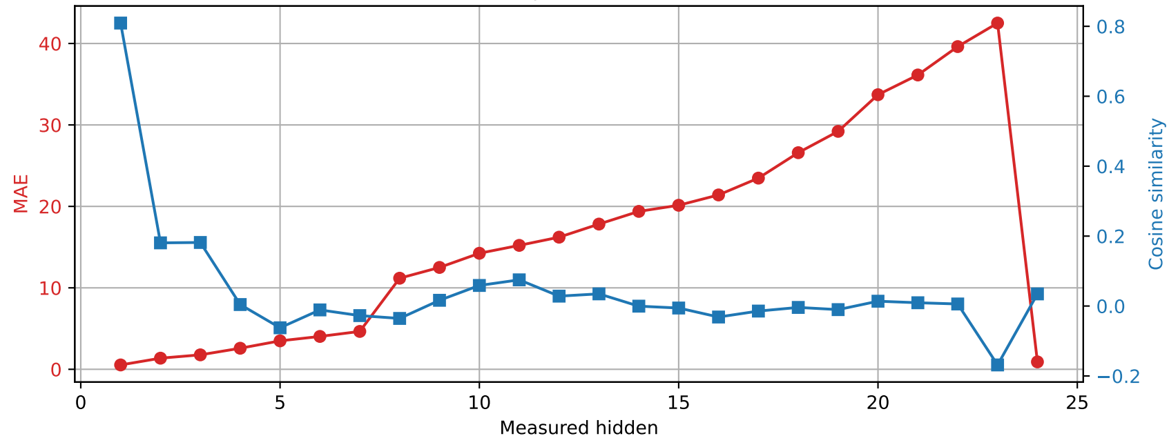
SmolLM2-1.7B-Instruct | Prompt 0 Spared layer 1 | Unquantized vs hybrid
