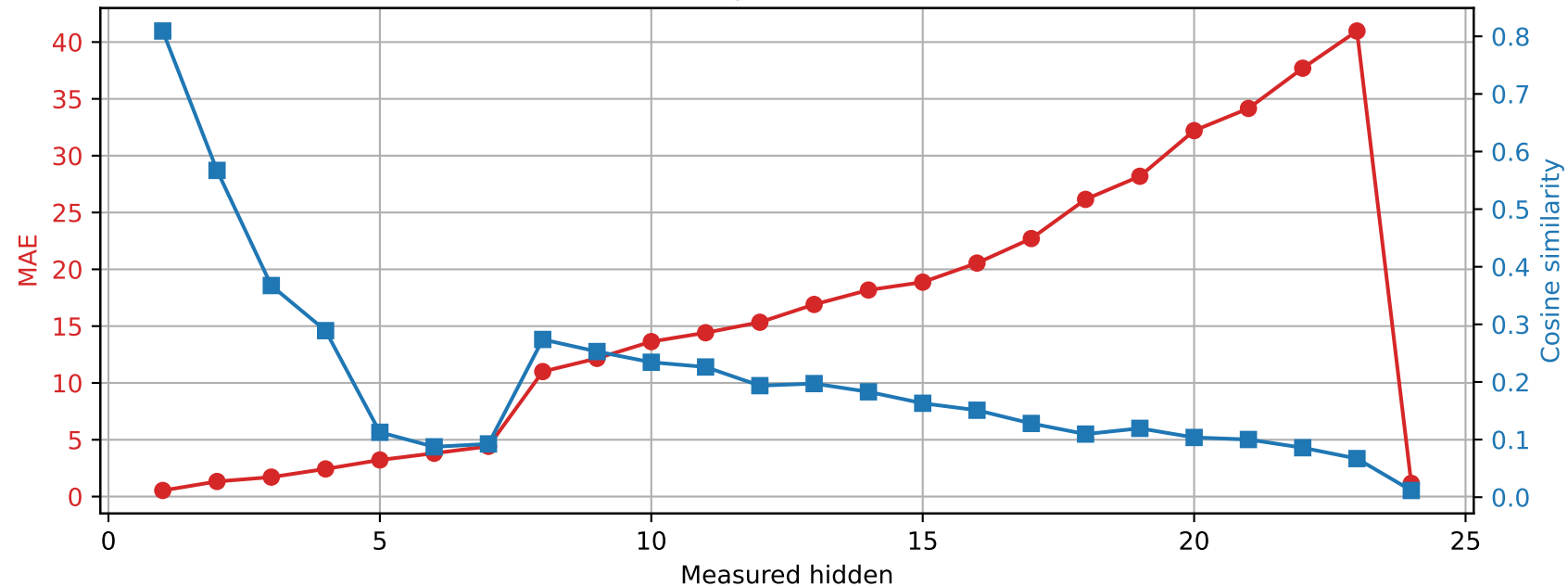
SmolLM2-1.7B-Instruct | Prompt 0 Spared layer 22 | Unquantized vs hybrid
