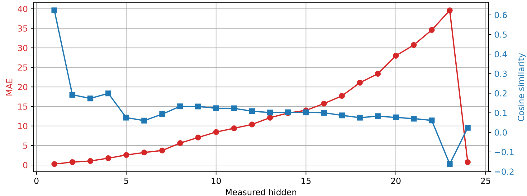
SmolLM2-1.7B-Instruct | Prompt 1 Spared layer 15 | Unquantized vs hybrid
