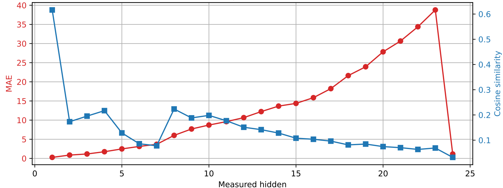
SmolLM2-1.7B-Instruct | Prompt 2 Spared layer 8 | Unquantized vs hybrid
