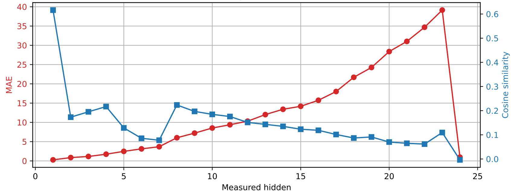
SmolLM2-1.7B-Instruct | Prompt 2 Spared layer 19 | Unquantized vs hybrid
