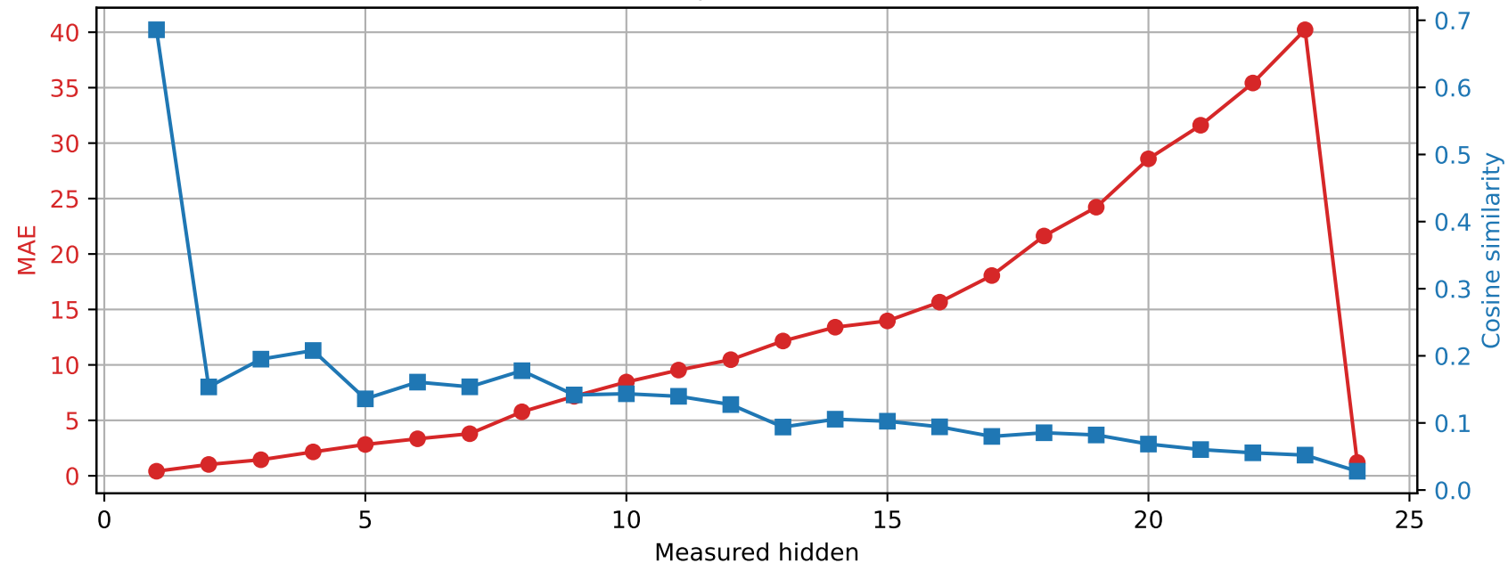
SmolLM2-1.7B-Instruct | Prompt 3 Spared layer 3 | Unquantized vs hybrid
