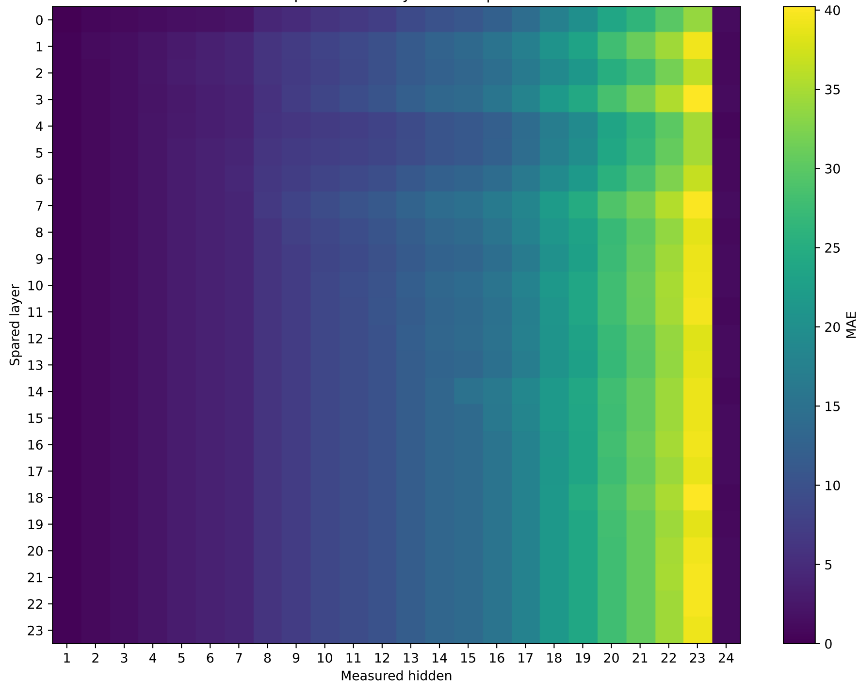
SmolLM2-1.7B-Instruct | Prompt 3 Unquantized vs hybrid MAE | int4
