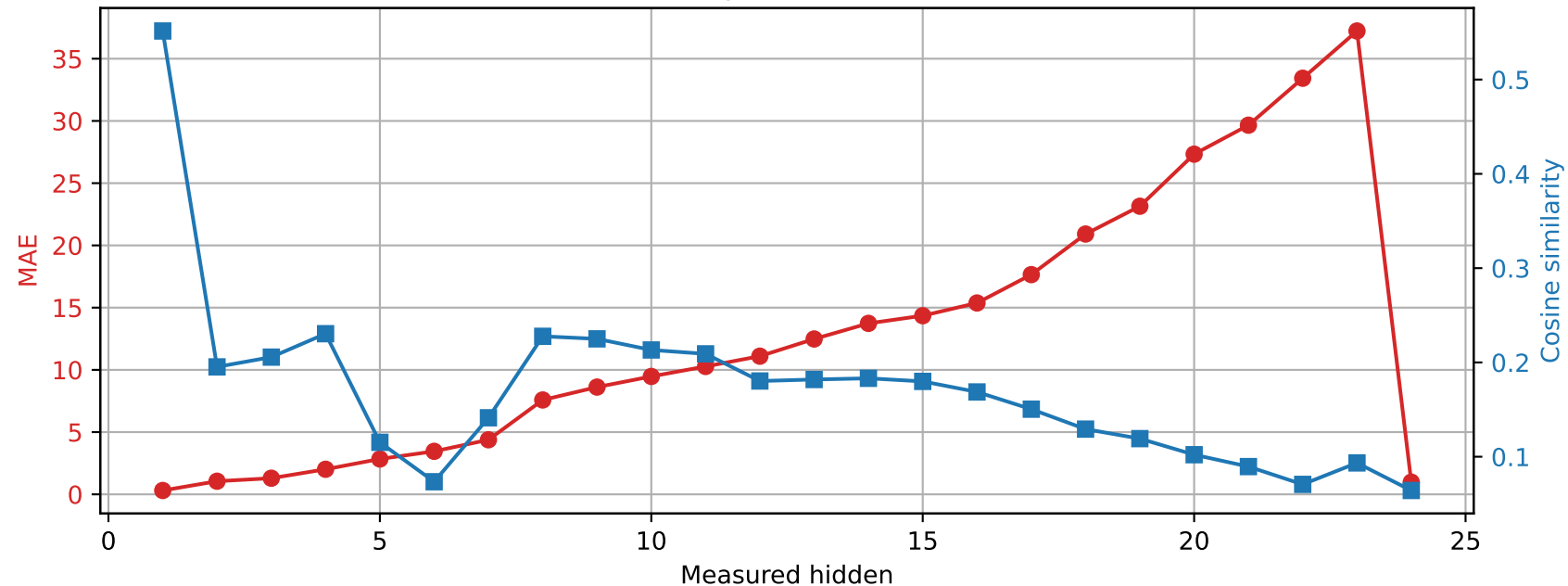
SmolLM2-1.7B-Instruct | Prompt 4 Spared layer 6 | Unquantized vs hybrid
