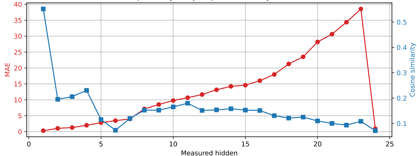
SmolLM2-1.7B-Instruct | Prompt 4 Spared layer 9 | Unquantized vs hybrid
