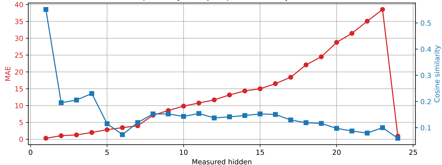
SmolLM2-1.7B-Instruct | Prompt 4 Spared layer 19 | Unquantized vs hybrid
