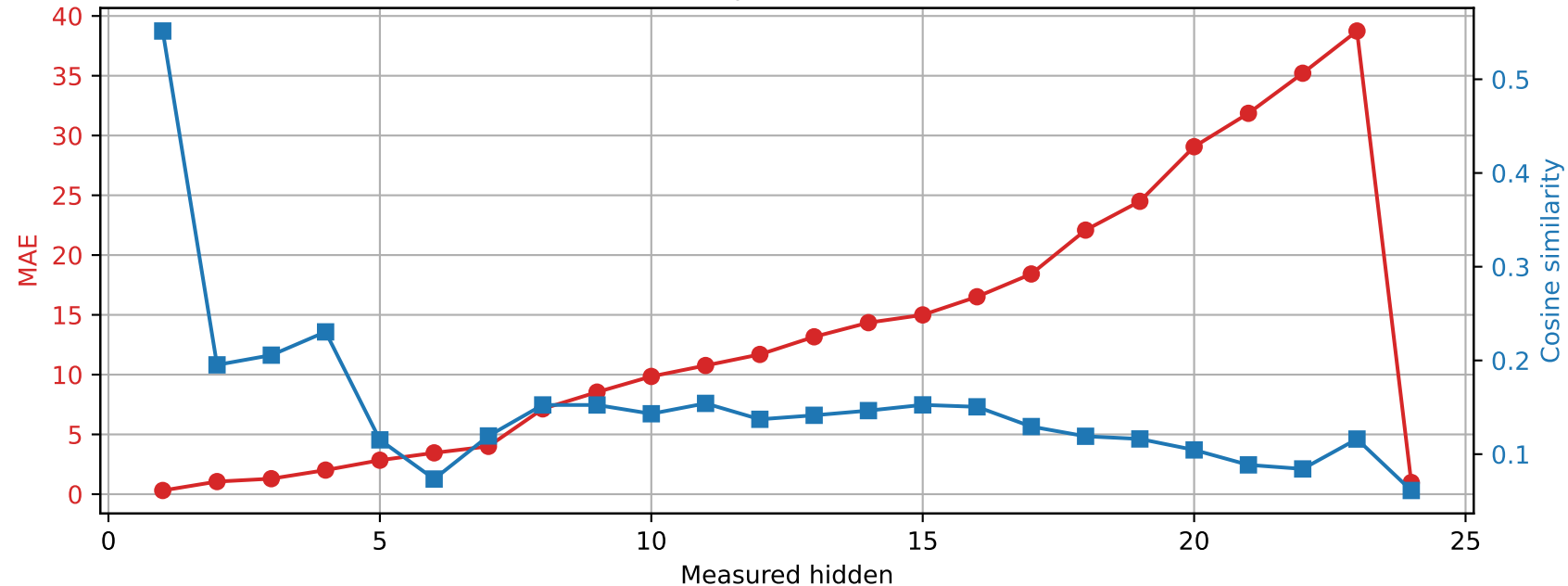
SmolLM2-1.7B-Instruct | Prompt 4 Spared layer 20 | Unquantized vs hybrid
