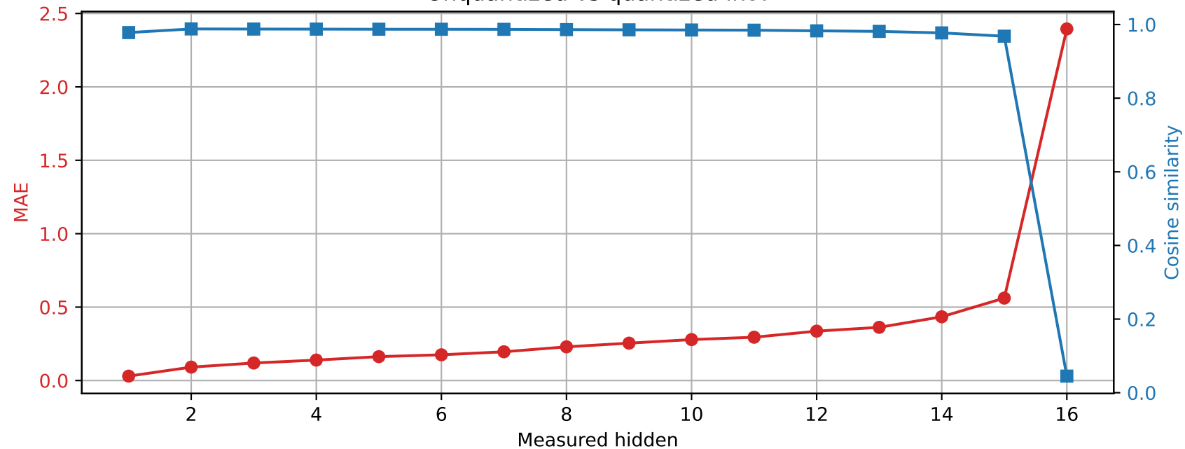
Llama-3.2-1B | Prompt 3 Unquantized vs quantized int4
