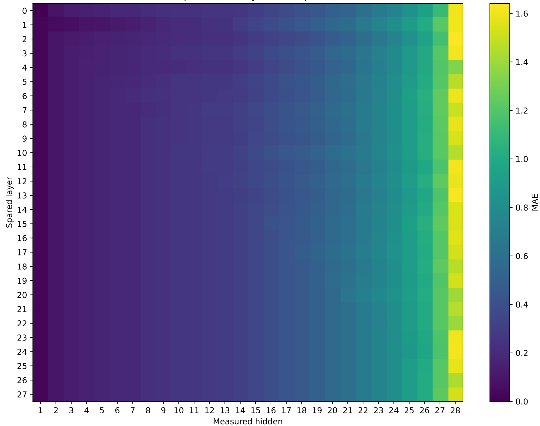
Llama-3.2-3B | Prompt 4 Unquantized vs hybrid MAE | int4
