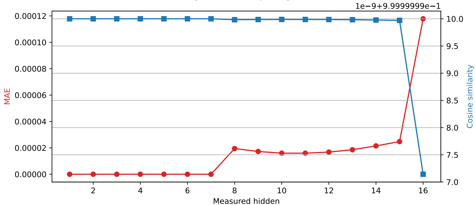
Llama-3.2-1B | Quantized layer 7 | float32 → int16
