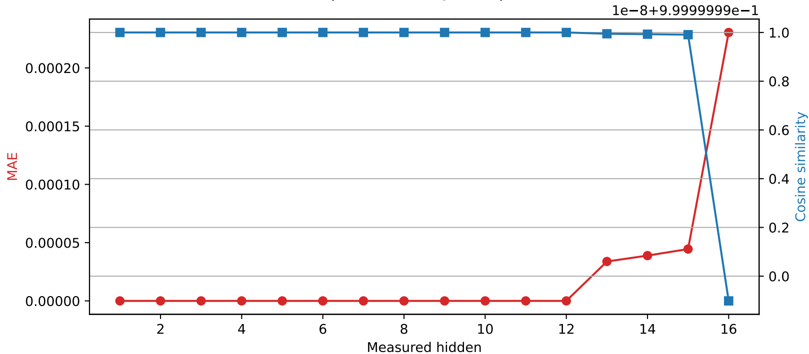
Llama-3.2-1B | Quantized layer 12 | float32 \rightarrow int16
