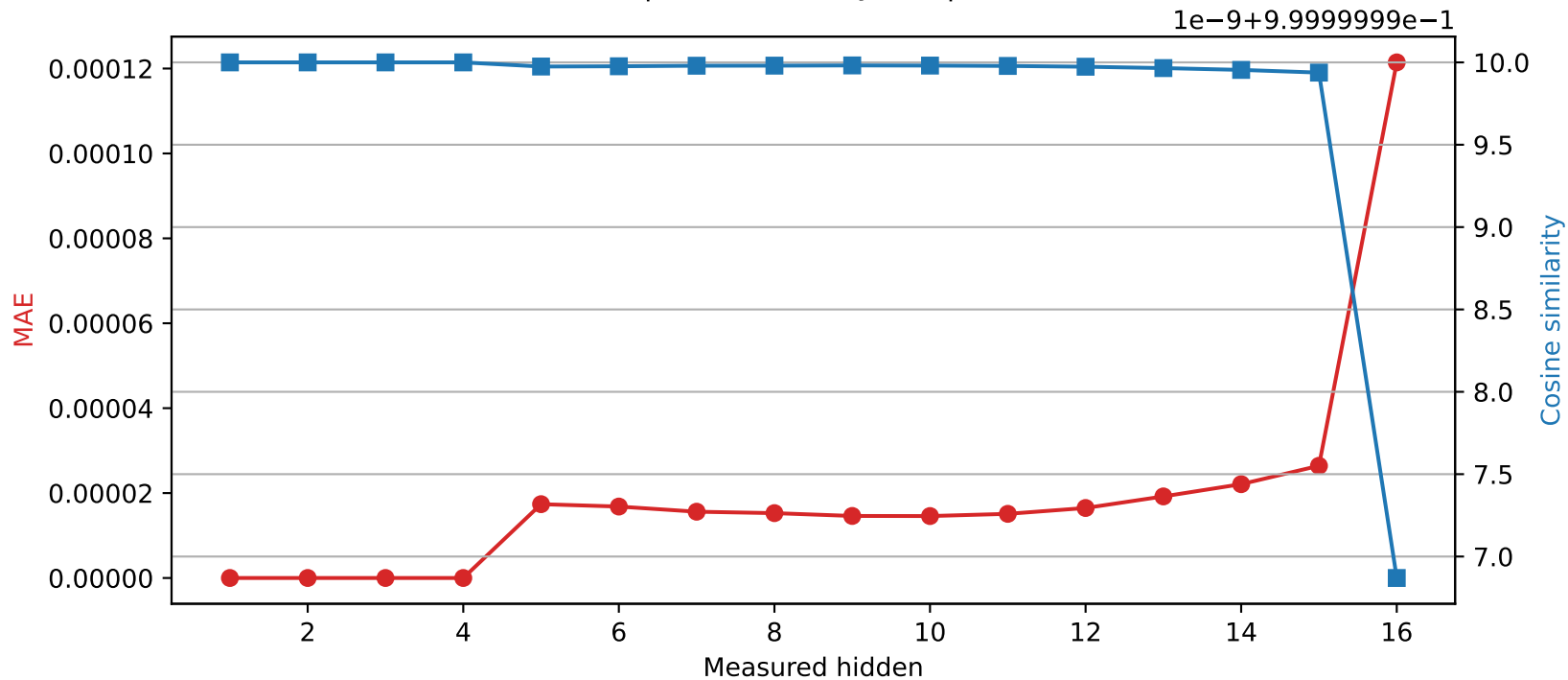
Llama-3.2-1B | Quantized layer 4 | float32 → int16
