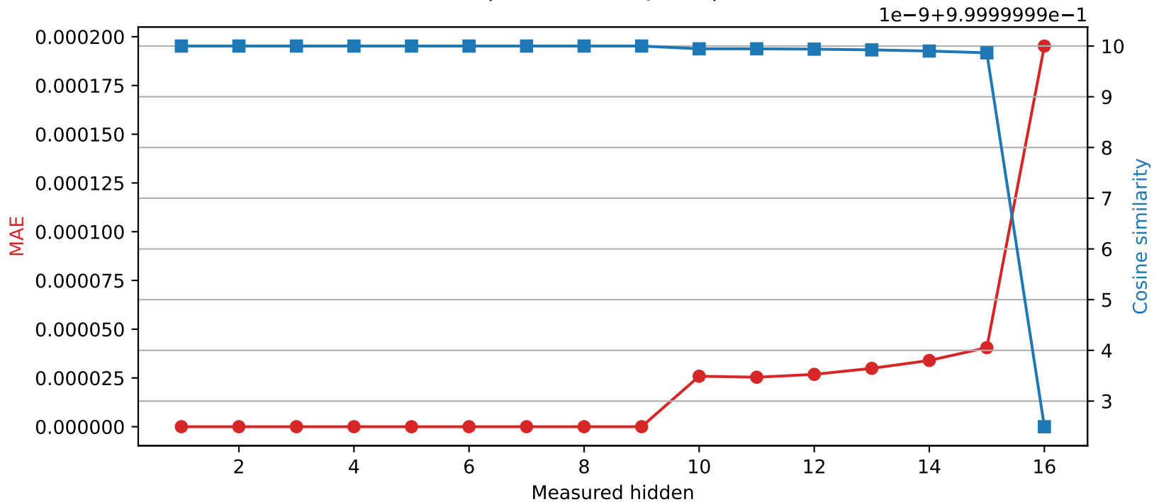
Llama-3.2-1B | Quantized layer 9 | float32 \rightarrow int16
