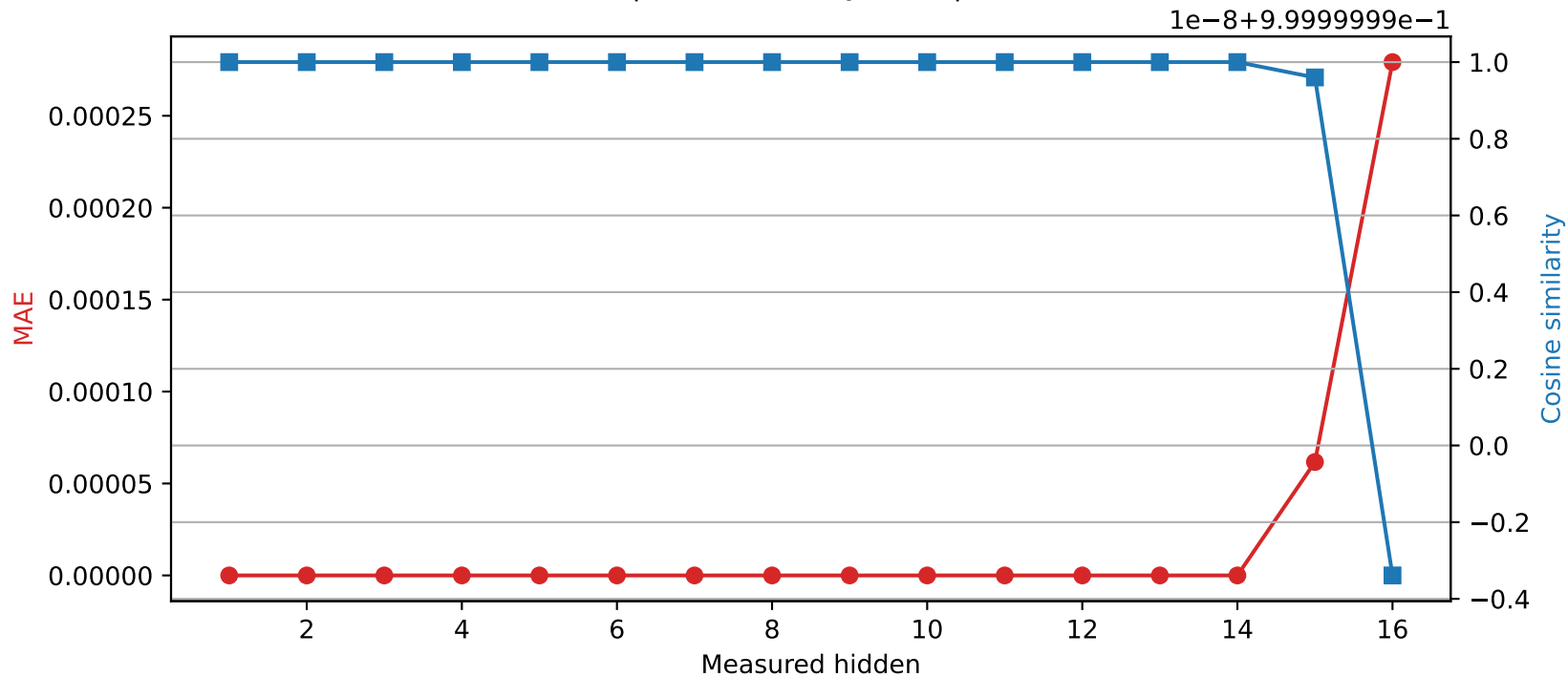
Llama-3.2-1B | Quantized layer 14 | float32 \rightarrow int16
