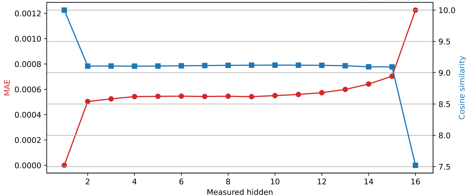
Llama-3.2-1B | Quantized layer 1 | float32 \rightarrow int16 1e-7+9.99999e-1
