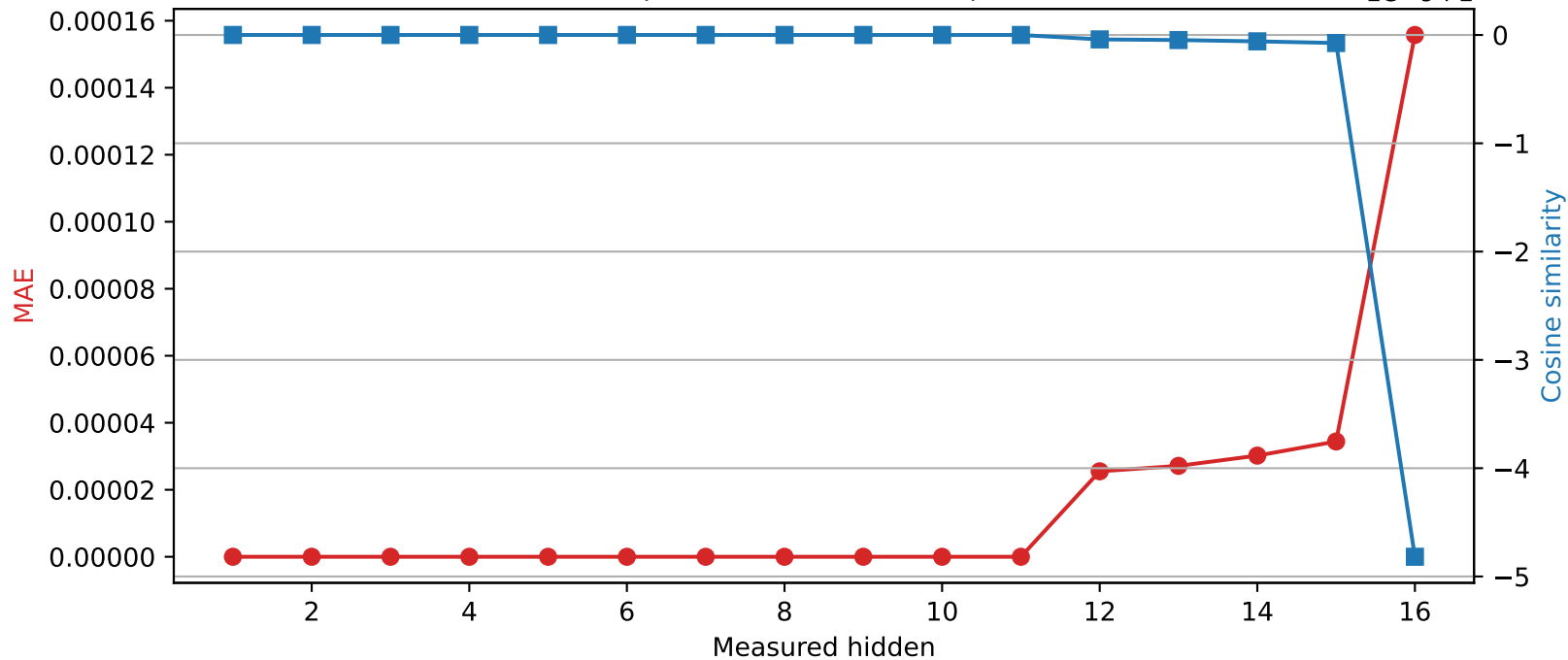
Llama-3.2-1B | Quantized layer 11 | float32 → int16
