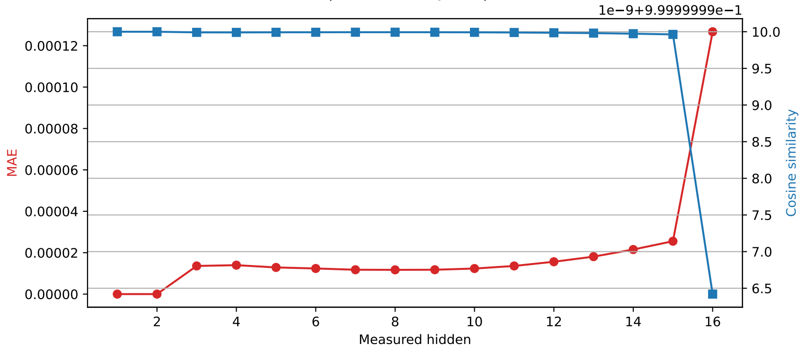
Llama-3.2-1B | Quantized layer 2 | float64 → int16
