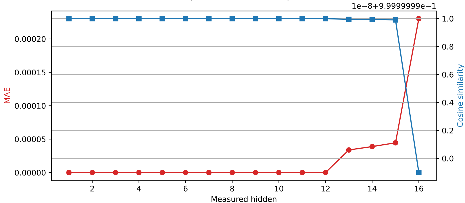
Llama-3.2-1B | Quantized layer 12 | float64 → int16
