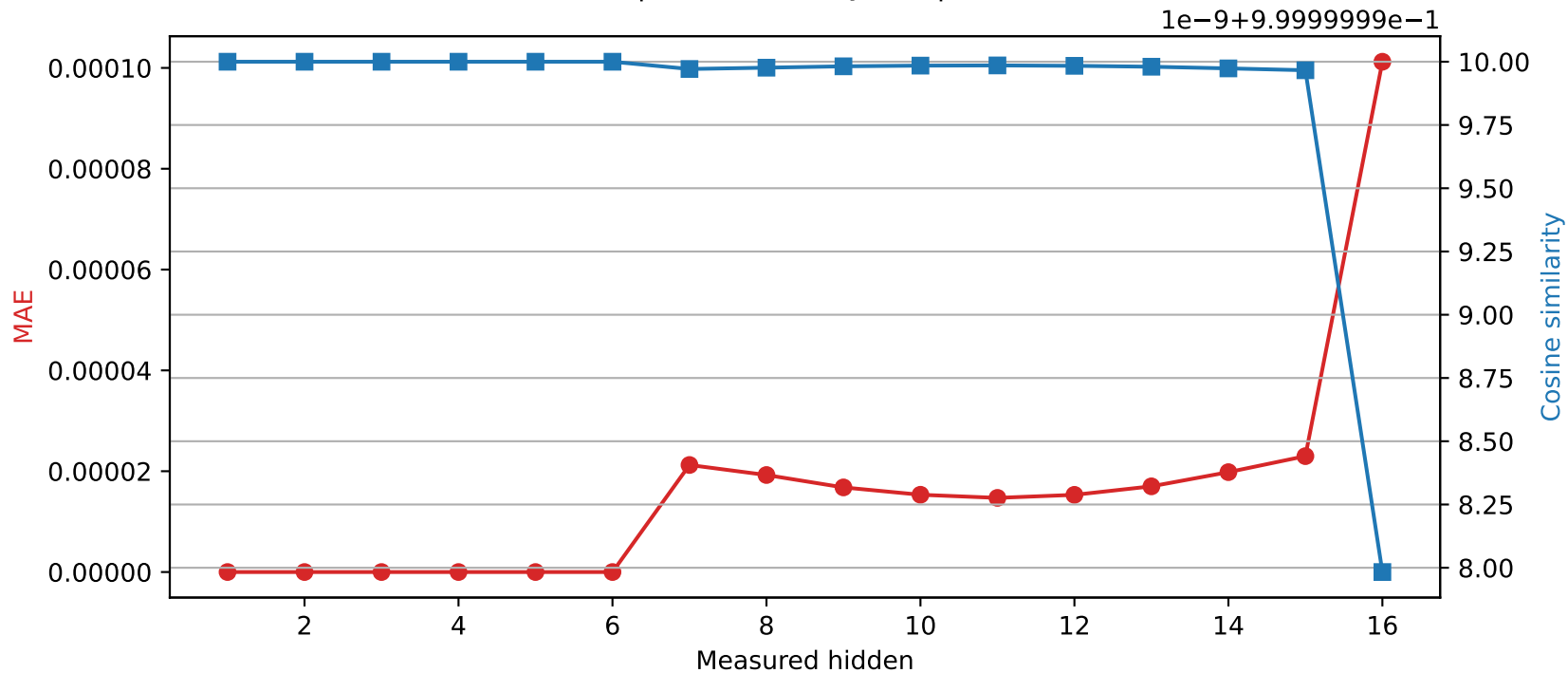
Llama-3.2-1B | Quantized layer 6 | float64 → int16
