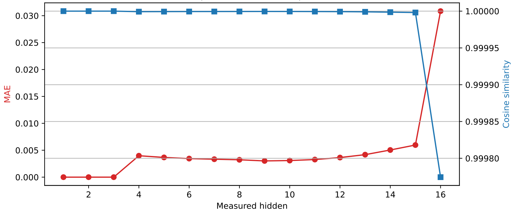
Llama-3.2-1B | Quantized layer 3 | float16 \rightarrow int8
