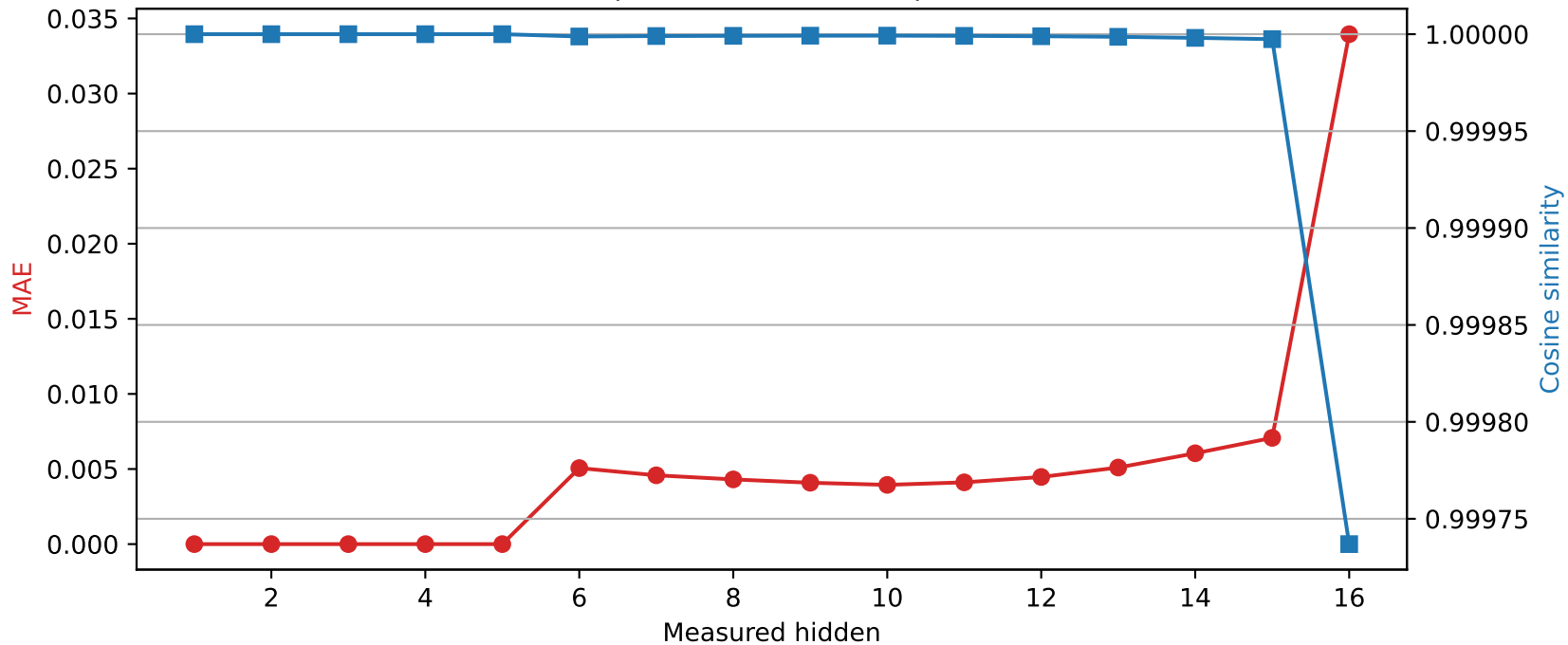
Llama-3.2-1B | Quantized layer 5 | float16 \rightarrow int8
