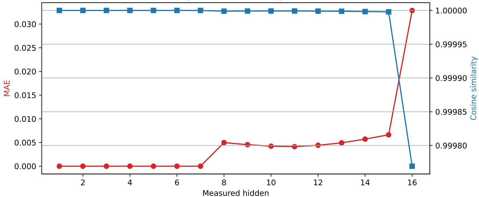
Llama-3.2-1B | Quantized layer 7 | float16 \rightarrow int8
