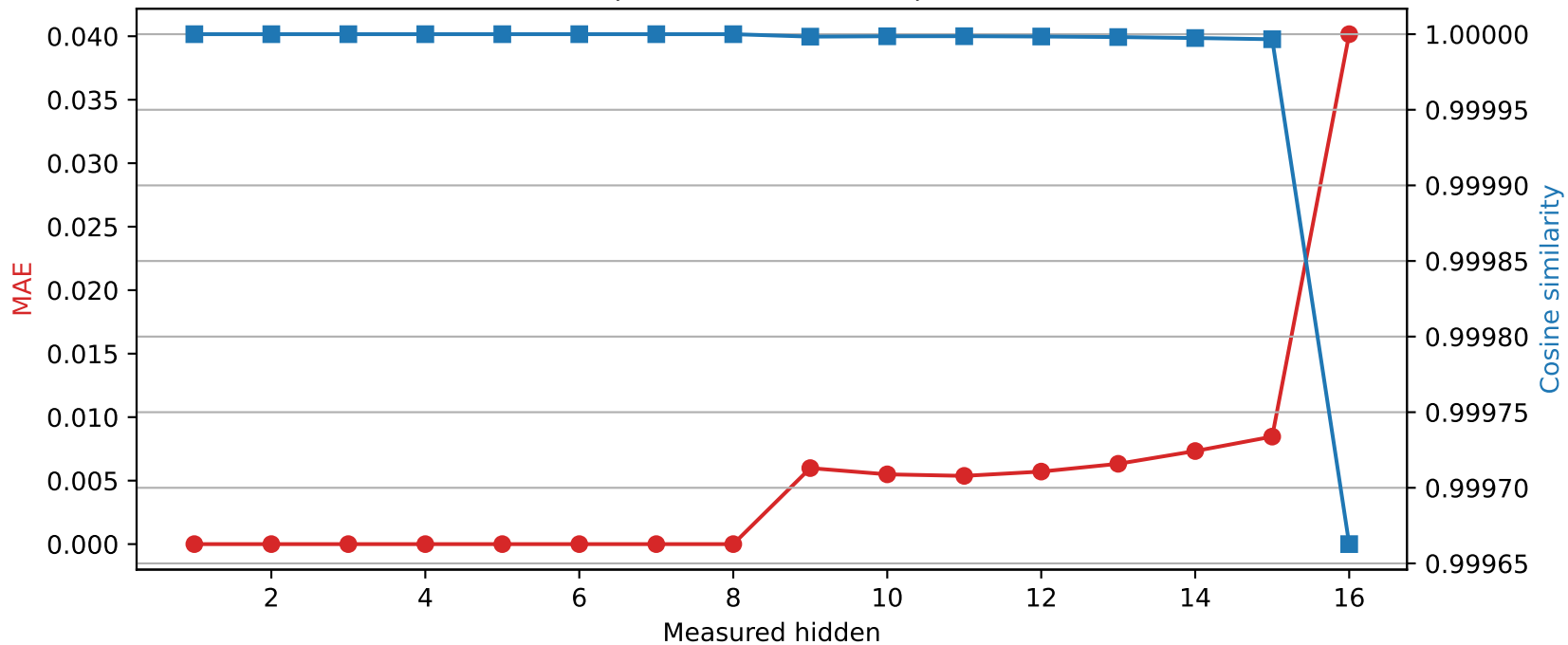
Llama-3.2-1B | Quantized layer 8 | float16 → int8
