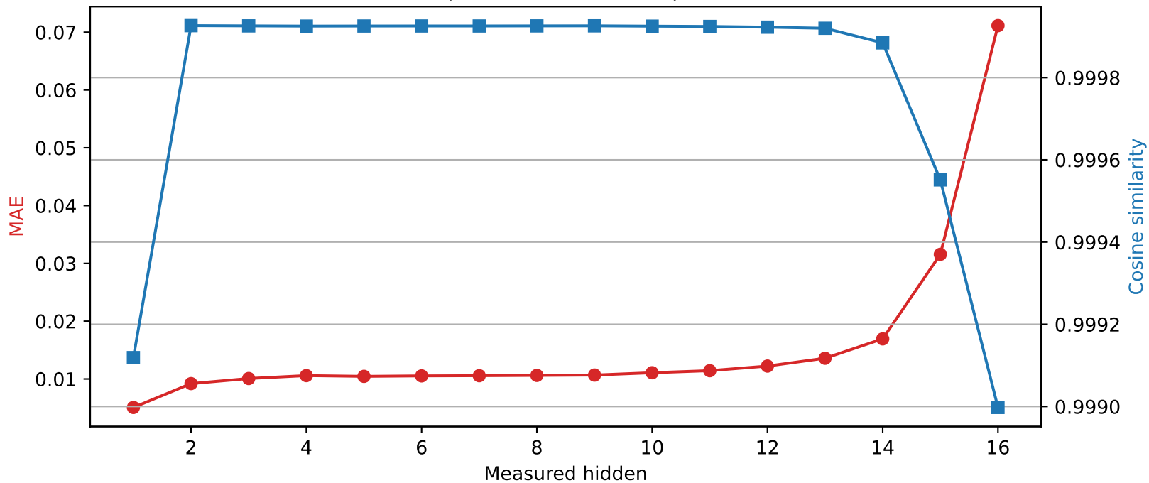
Llama-3.2-1B | Quantized layer 0 | float16 \rightarrow int8
