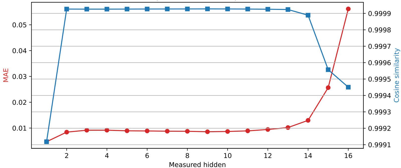
Llama-3.2-1B | Quantized layer 0 | float16 → int8
