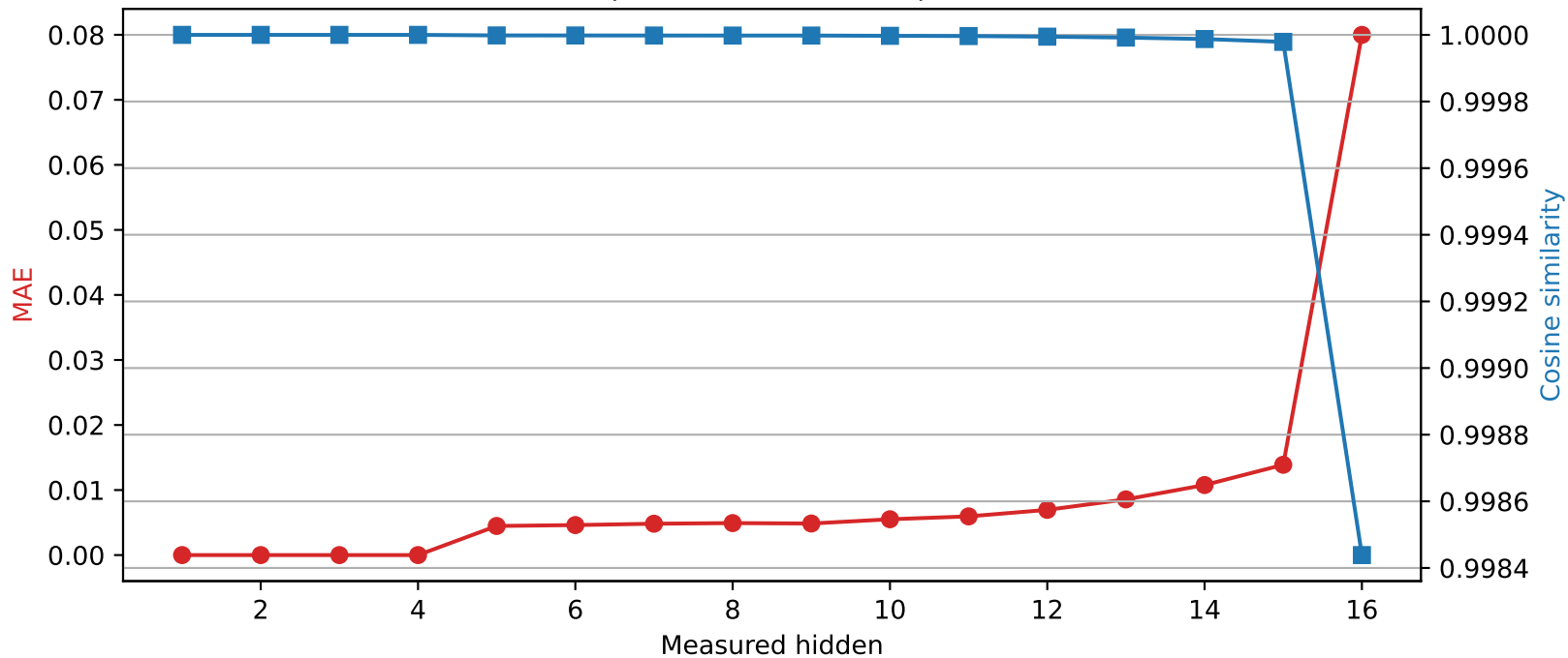
Llama-3.2-1B | Quantized layer 4 | float16 → int8
