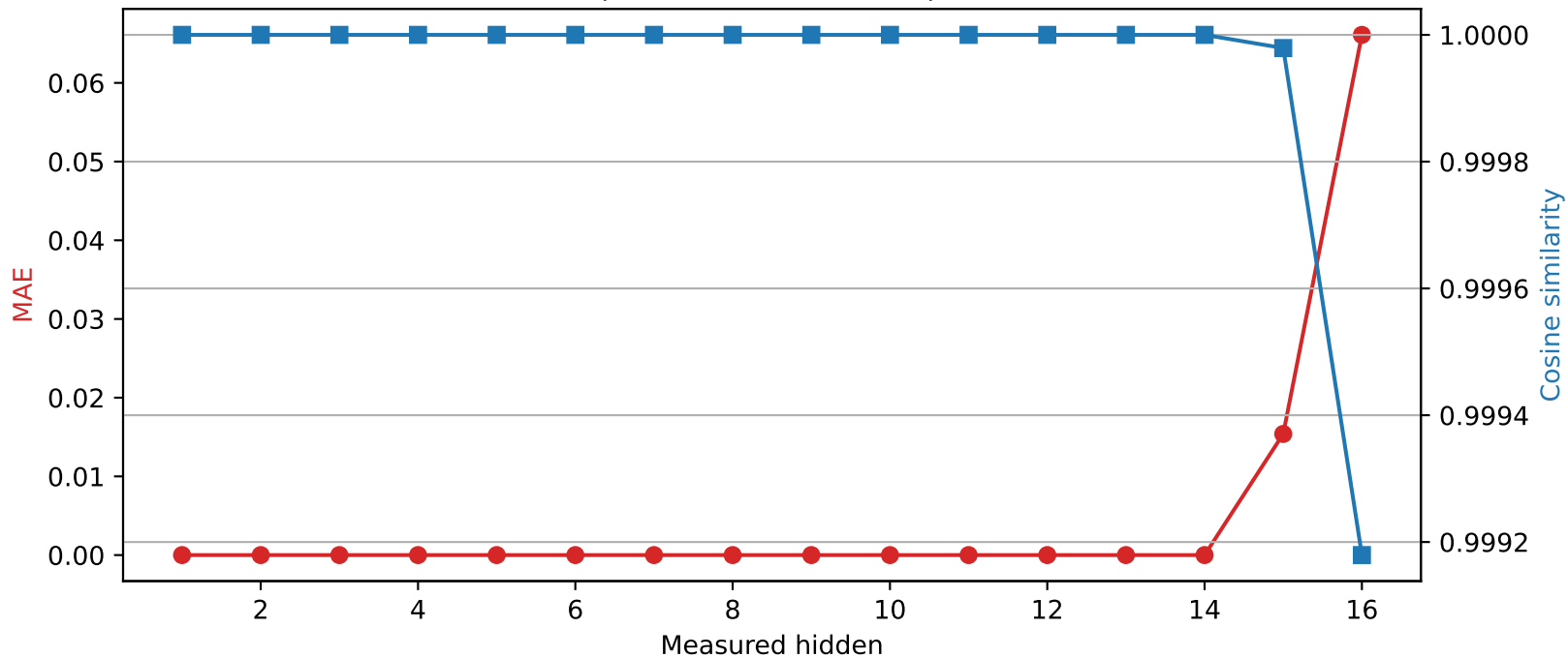
Llama-3.2-1B | Quantized layer 14 | float16 \rightarrow int8
