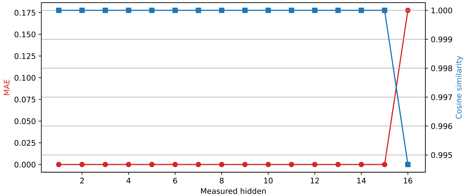
Llama-3.2-1B | Quantized layer 15 | float16 \rightarrow int8
