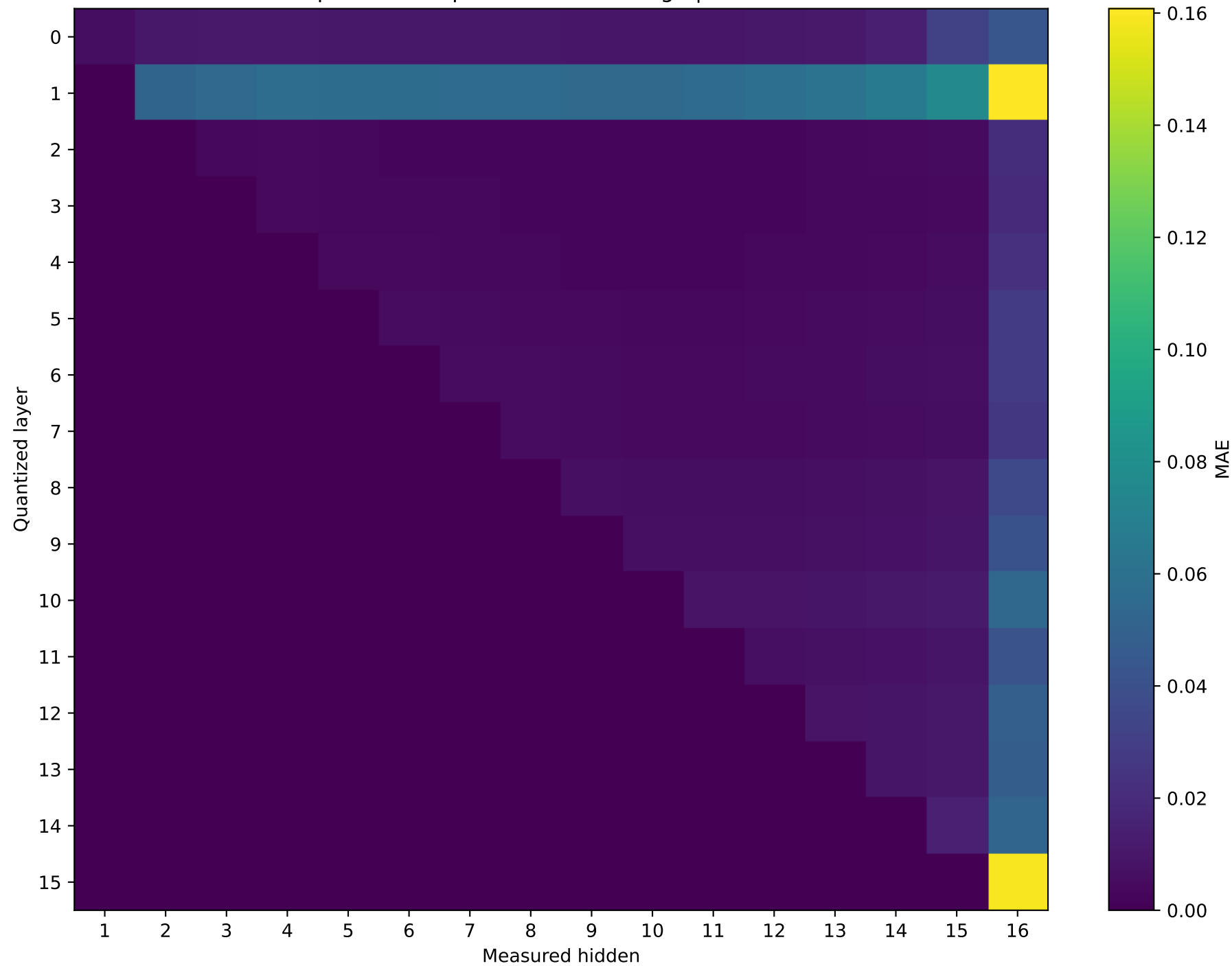
Llama-3.2-1B Prompt 4: MAE representation damage | float16 → int8
