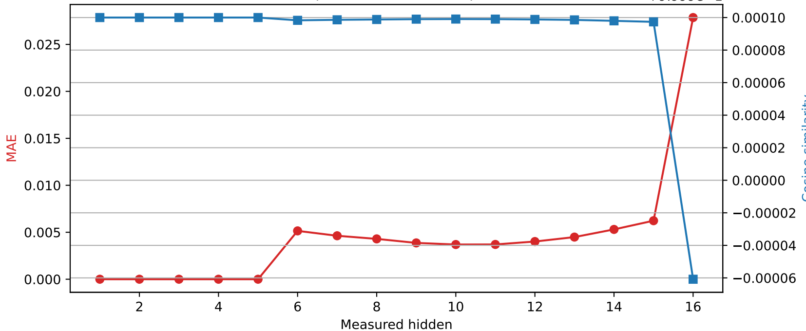
Llama-3.2-1B | Quantized layer 5 | float16 → int8
