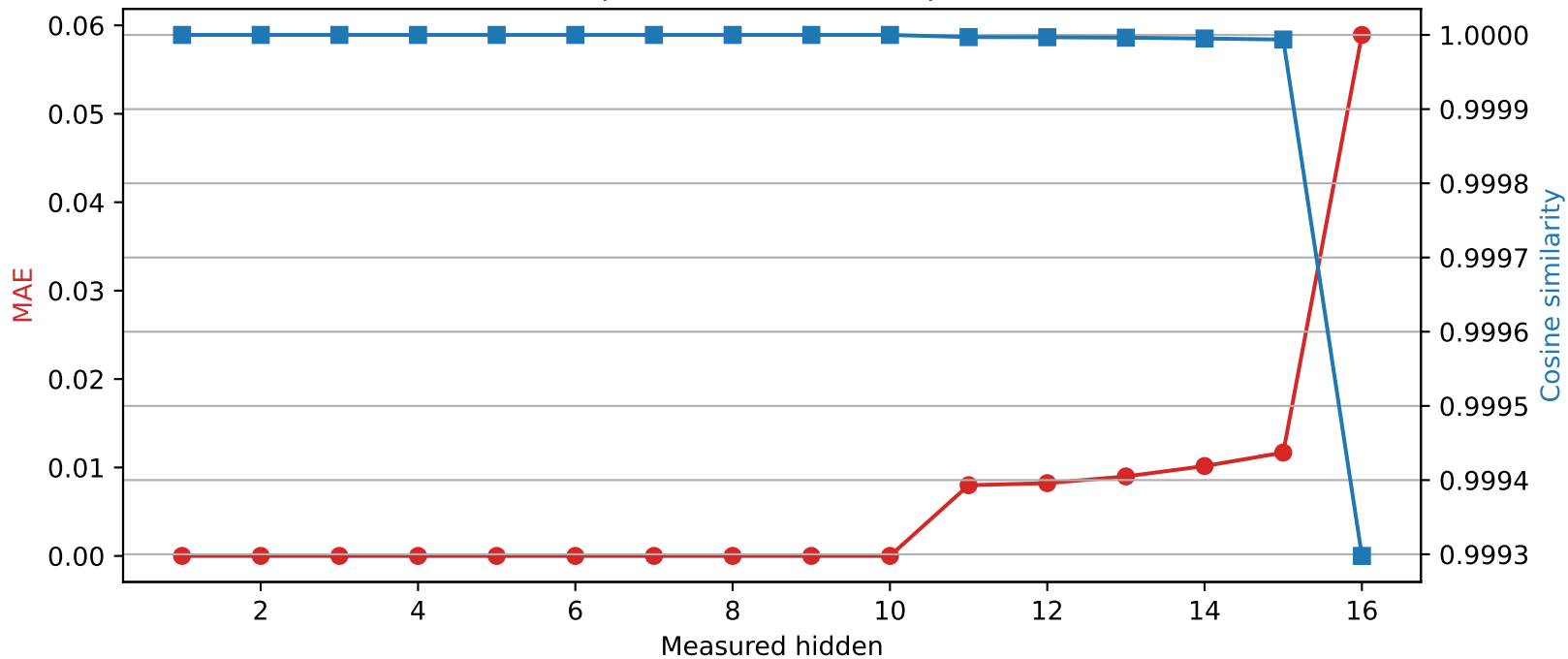
Llama-3.2-1B | Quantized layer 10 | float32 → int8
