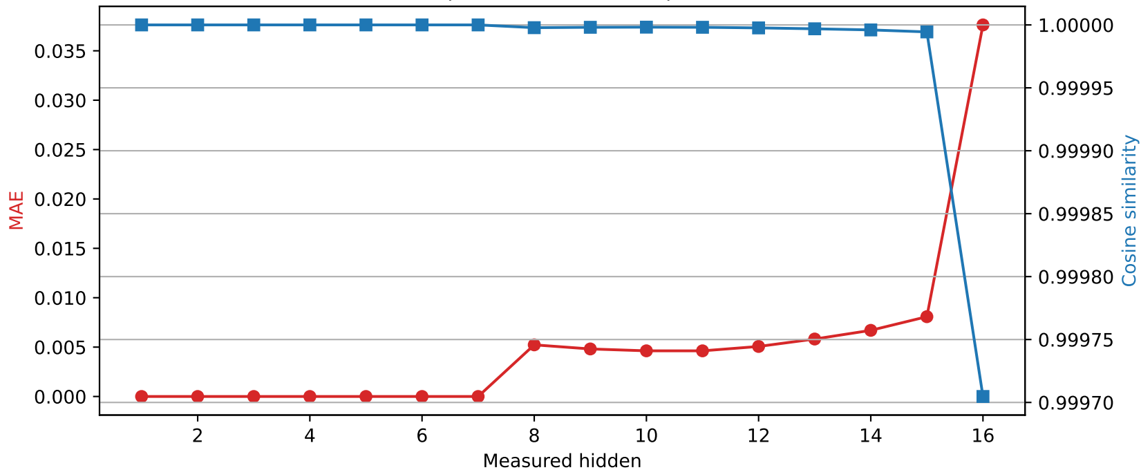
Llama-3.2-1B | Quantized layer 7 | float32 → int8
