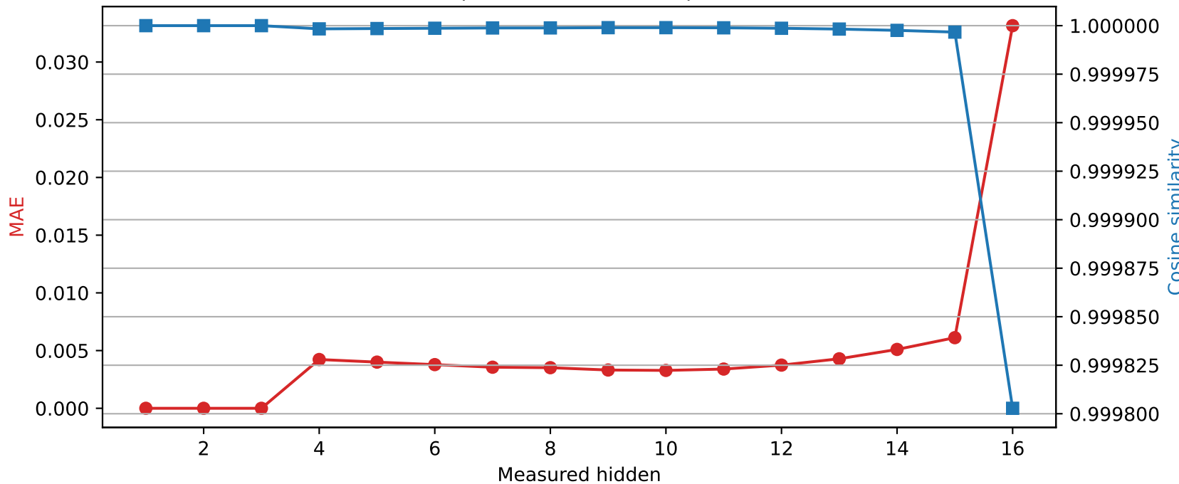
Llama-3.2-1B | Quantized layer 3 | float32 → int8
