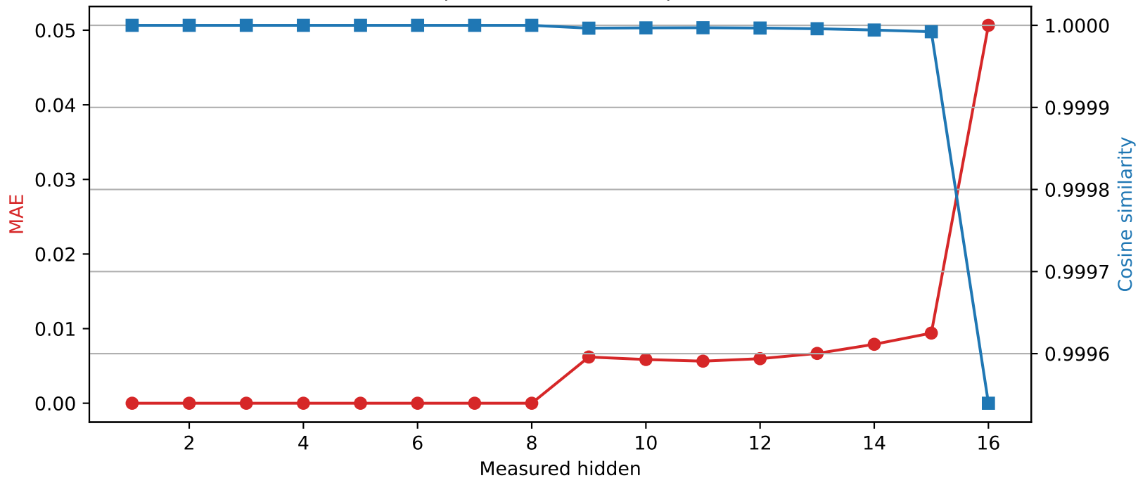
Llama-3.2-1B | Quantized layer 8 | float32 → int8
