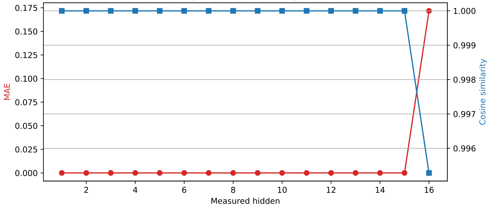
Llama-3.2-1B | Quantized layer 15 | float32 → int8
