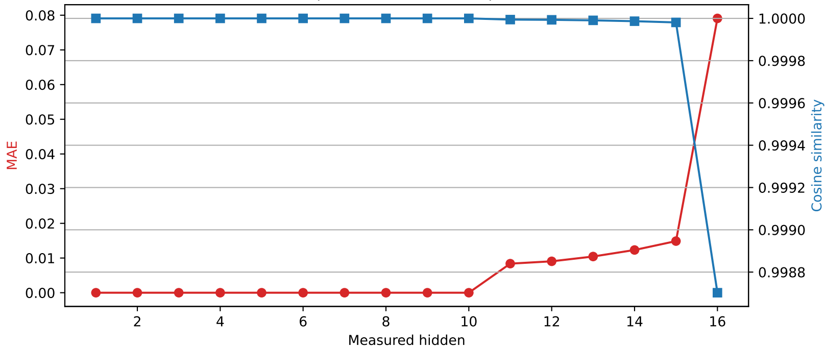
Llama-3.2-1B | Quantized layer 10 | float32 \rightarrow int8
