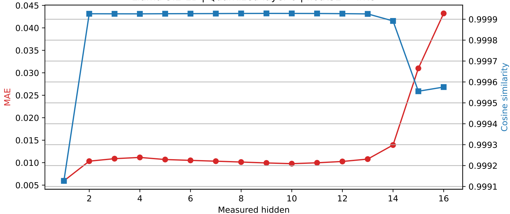
Llama-3.2-1B | Quantized layer 0 | float32 \rightarrow int8
