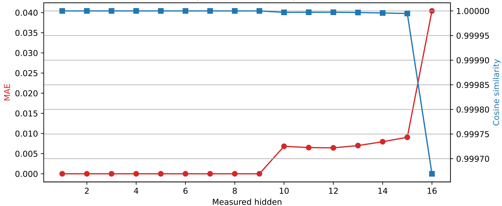
Llama-3.2-1B | Quantized layer 9 | float32 → int8
