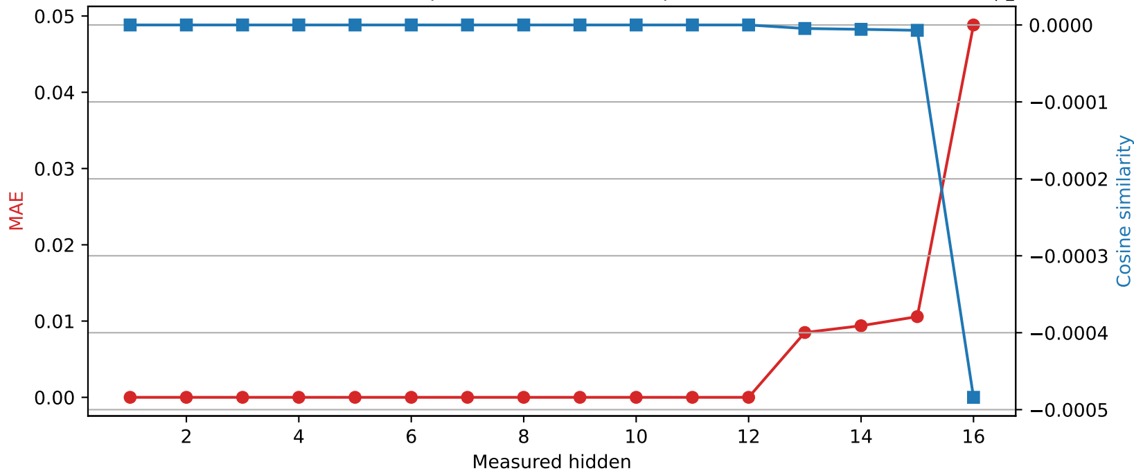
Llama-3.2-1B | Quantized layer 12 | float32 \rightarrow int8
