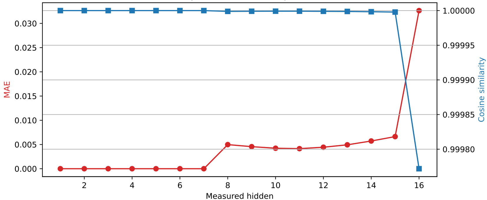
Llama-3.2-1B | Quantized layer 7 | float64 \rightarrow int8
