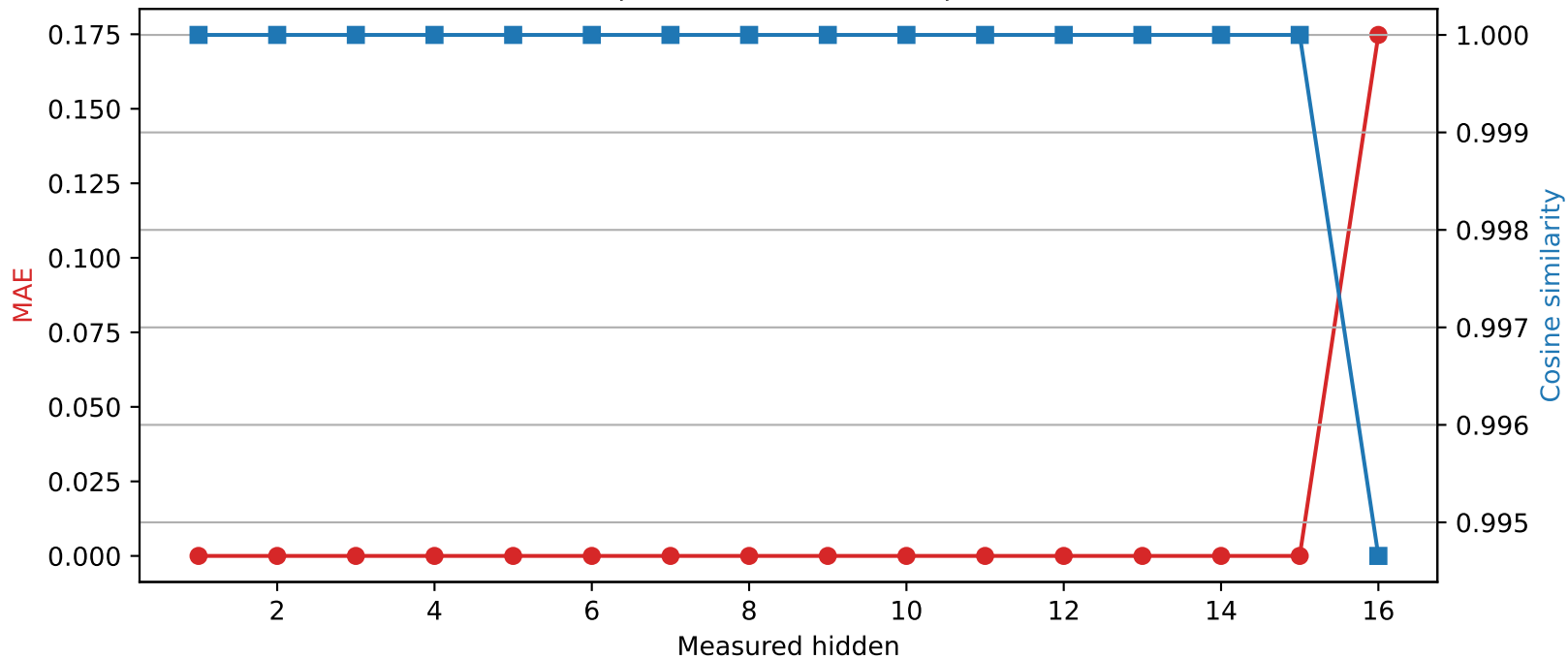
Llama-3.2-1B | Quantized layer 15 | float64 → int8
