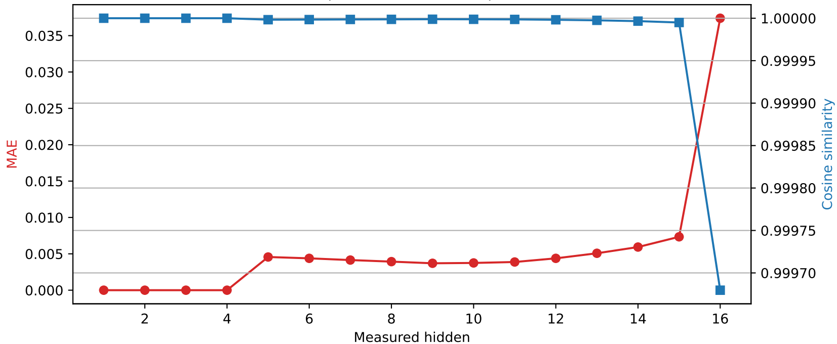
Llama-3.2-1B | Quantized layer 4 | float64 → int8
